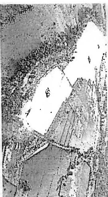
Waterfilled- Aerial photographs- Krishnakuppam Manakollai waterbody
