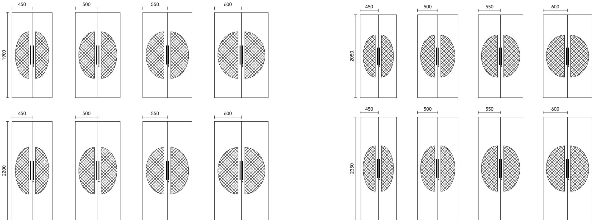
Dimension Detail (in mm)
