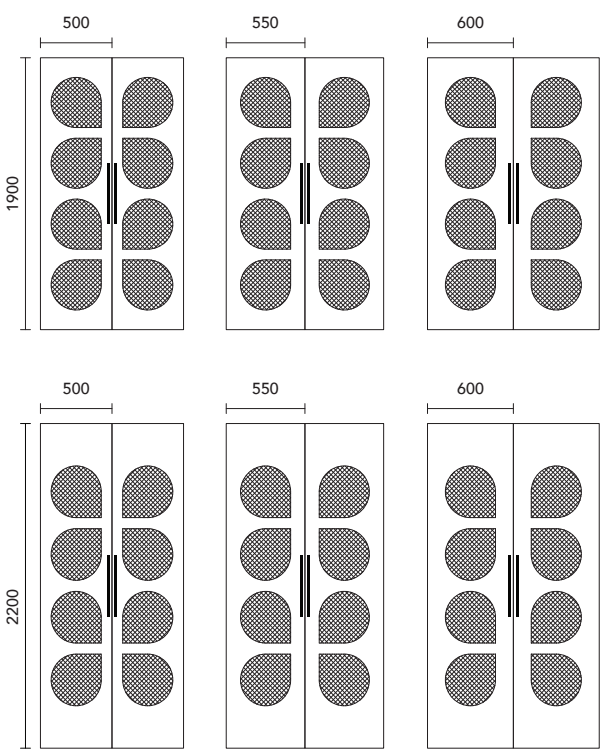
Dimension Detail (in mm)
